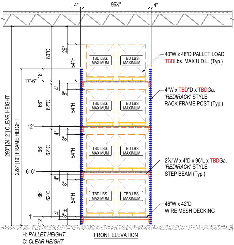
A2 RACKING ELEVATIONS (TYP.) SCALE: 1/40
