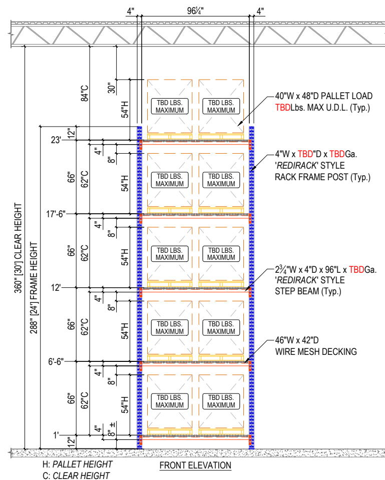
A1 RACKING ELEVATIONS (TYP.)
